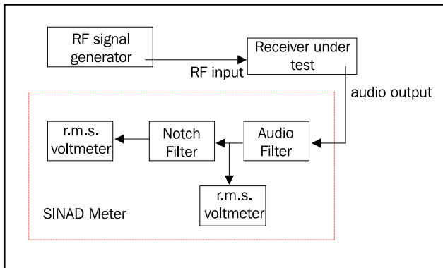
Figure 1.- SINAD measurement system
