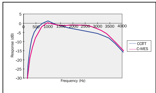
Figure 3 - Comparison of C-MES and CCITT Frequency Response
