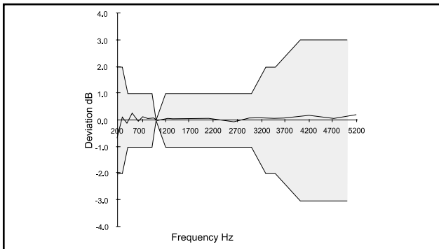
Figure 7 - Filter response compared to CMESSAGE standard error band
