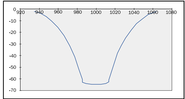
Figure 8 - Frequency response of the notch filter on 2023 series Option 12
