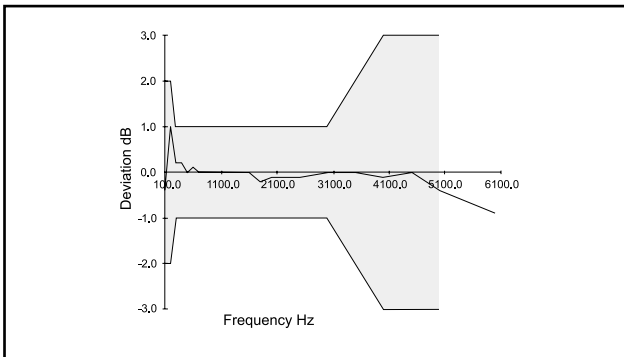
Figure 6 - Filter response compared to CCITT standard error band
