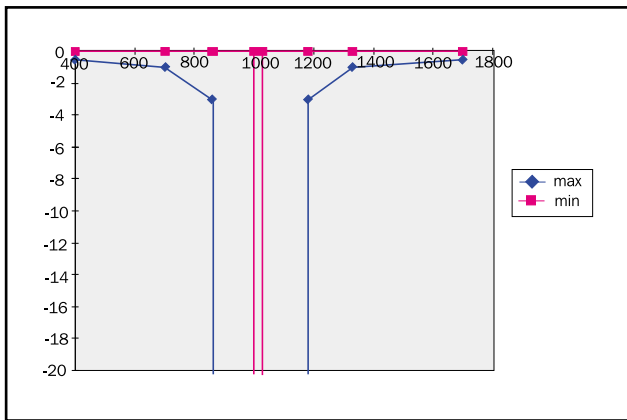
Figure 4 - Limits for Notch Filter ITU-T O.132
